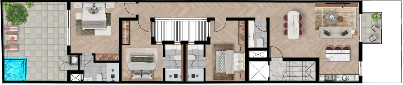
PROPOSED FIRST FLOOR PLAN SCALE: 1/8" = 1'-0"
