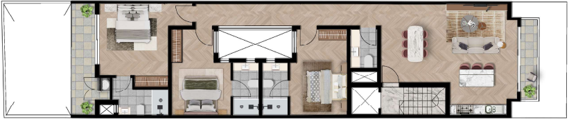
PROPOSED SECOND FLOOR PLAN SCALE: 1/8" = 1'-0"
